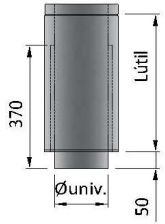
KWKVW EXTENSIBLE VITRIFICADO A KW DE 1 m CONNECTING PIPE STARTER LENGHT 1 m
