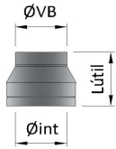
KWDV MANGUITO KW A VB ADAPTOR KW TO VB
