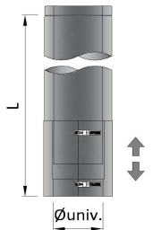
KWAT KW ADAPTADOR AJUSTABLE 1 m ADJUSTABLE CONNECTING PIPE 1 m
